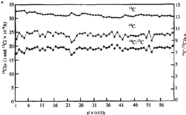
图 3 A-交替加速时, ^{13}\text{H} 、 ^{14}\text{C} 束流和 ^{14}\text{C}/^{13}\text{CH} 比值随测量循环次数的变化 Fig. 3 ^{14}\text{C} , ^{14}\text{C} and ^{14}\text{C}/^{13}\text{CH} versus cycle number during A-sequential acceleration where the maximum ^{14}\text{C} counting rate reached is about 25 cps measured in 60 cycles with each 40 s by consecutively rotating samples three times
